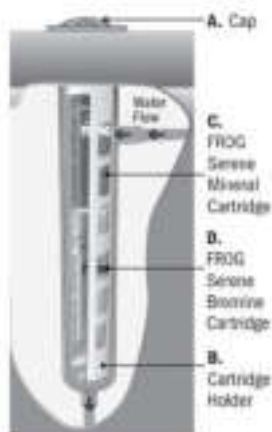
Cut-away view of cartridges strapped into holder and placed into the In-Line System.
