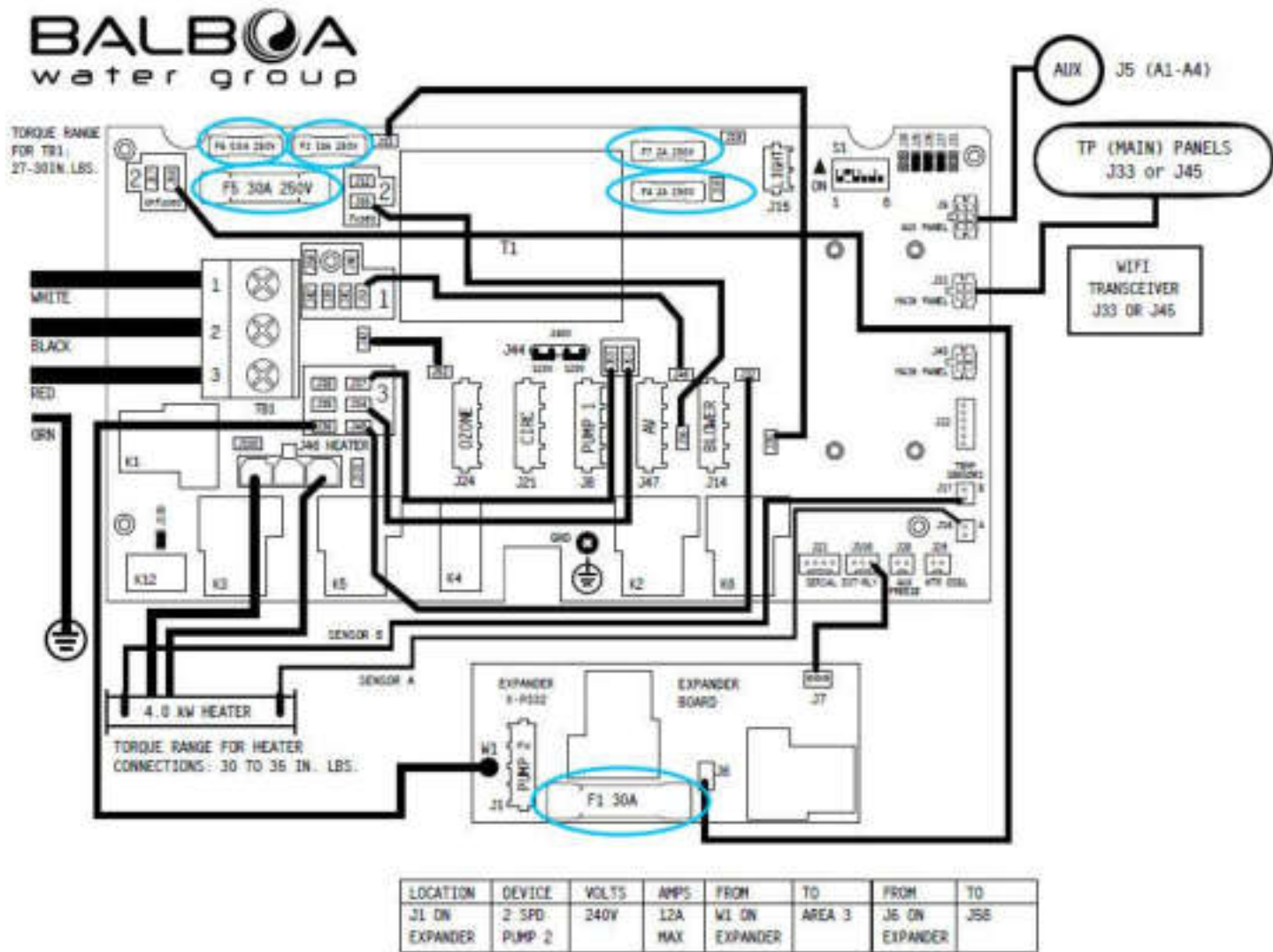
“Typical Board Layout”
